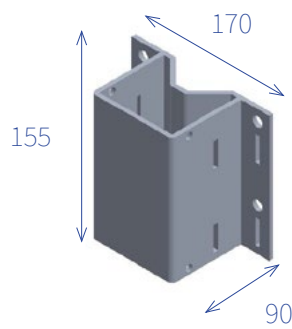
FIXATION POTEAU
